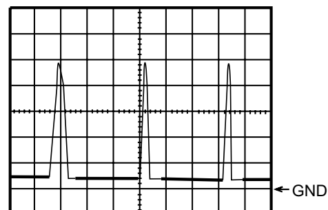
WF10 1DIV: 5V 20 \mu sec WH501A Pin 1
